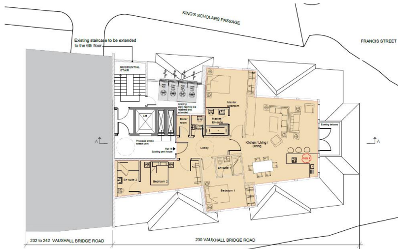
PROPOSED SIXTH FLOOR PLAN
