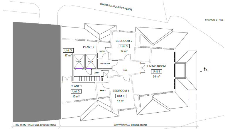
EXISTING SIXTH FLOOR PLAN
